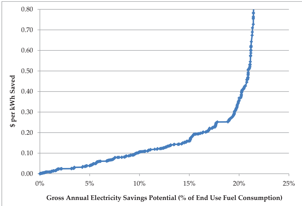
Figure 4-1. Sample Supply Curve of Gross Annual Electric Energy Savings Potential of Lighting in the Industrial Food Segment
