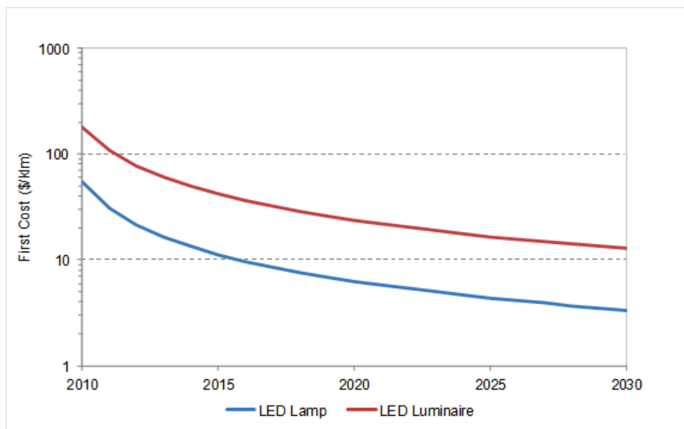
Figure 5-11. Forecasted LED Price ($/klm) Improvement
